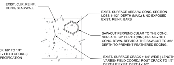
TYPE II REPAIR MODIFICATION
