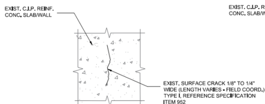
TYPE I REPAIR MODIFICATION
