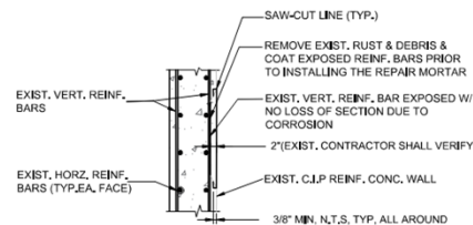
TYPE III REPAIR MODIFICATION
